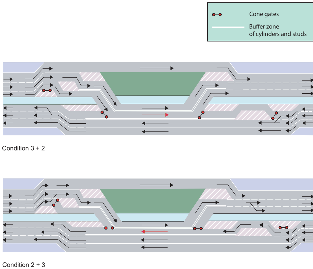
Figure 6.6 Schematic of tidal flow layout for partial contra-flow on three-lane carriageways
