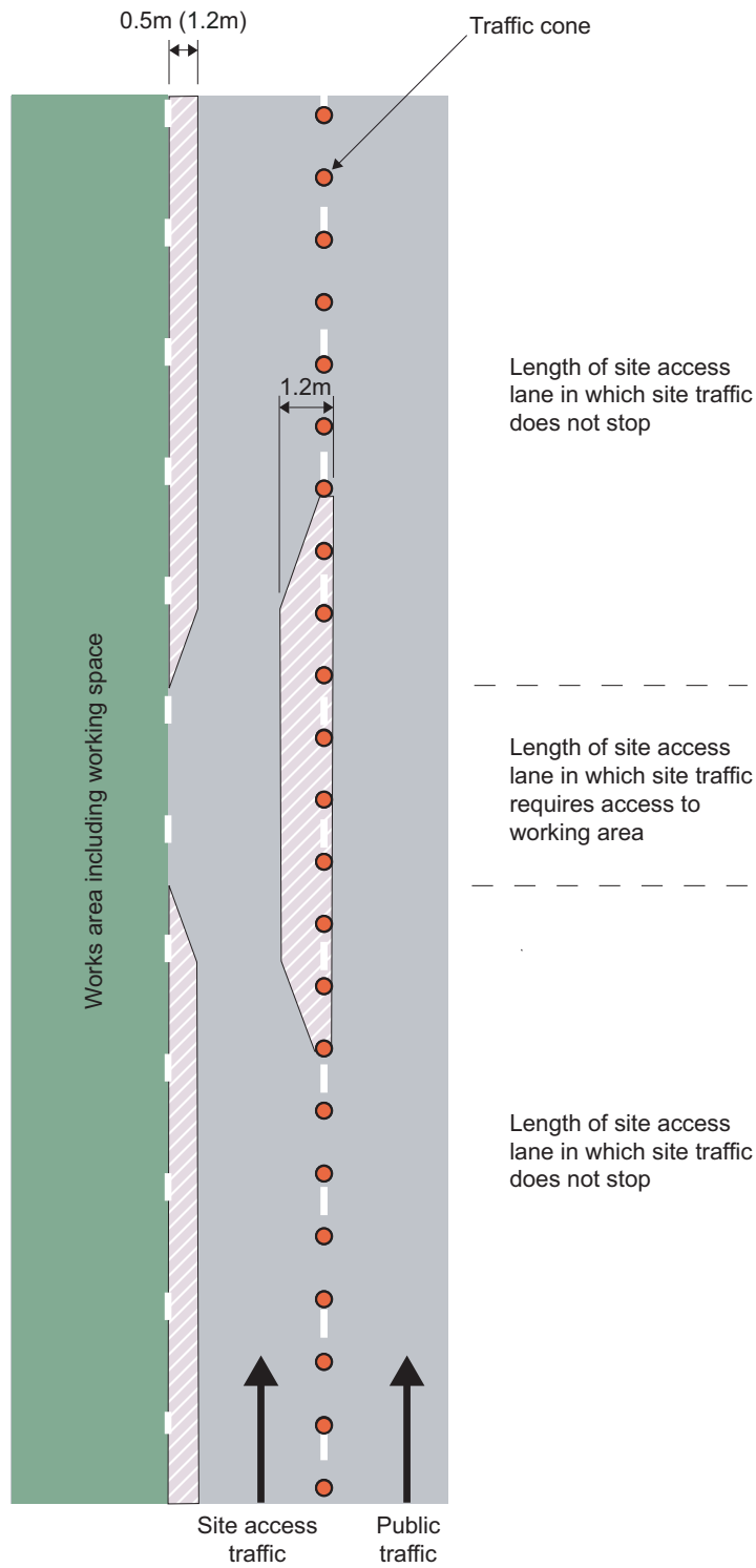
Figure 3.2 Location of safety zones in relation to site access lane
